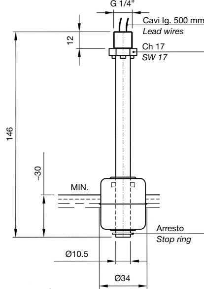
LEM5LANA NA CONTACT
