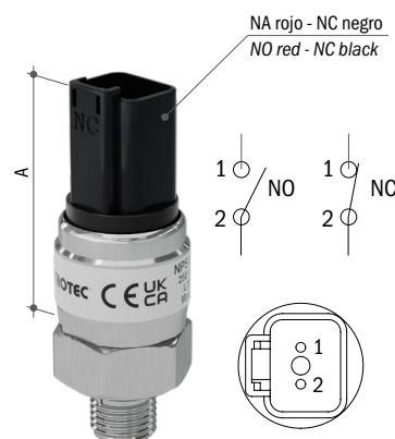
Deutsch DT04-2P NA normalmente abierto / NC normalmente cerrado NO normally open / NC normally closed
